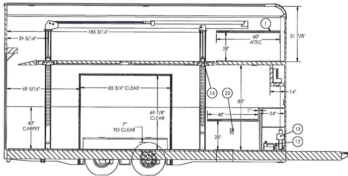
INTERIOR ROADSIDE SECTION B-B
