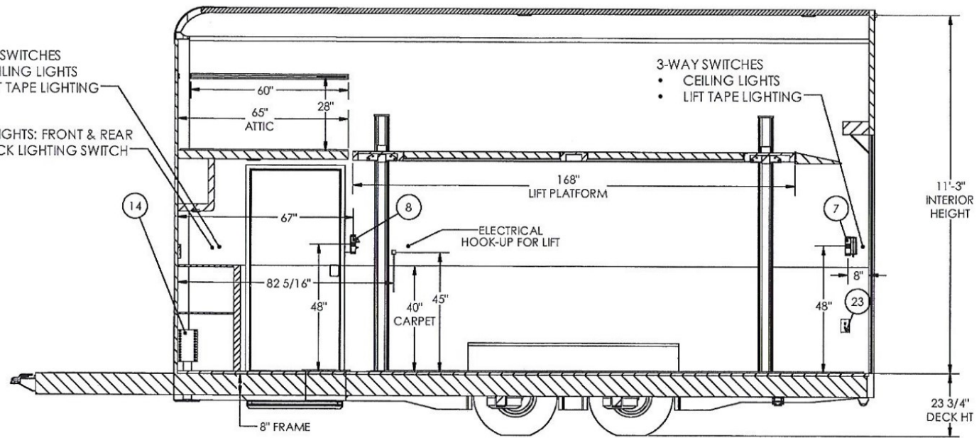
INTERIOR CURBSIDE SECTION A-A
